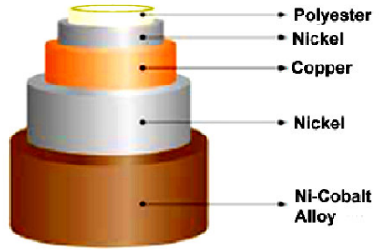
Thread Composition
